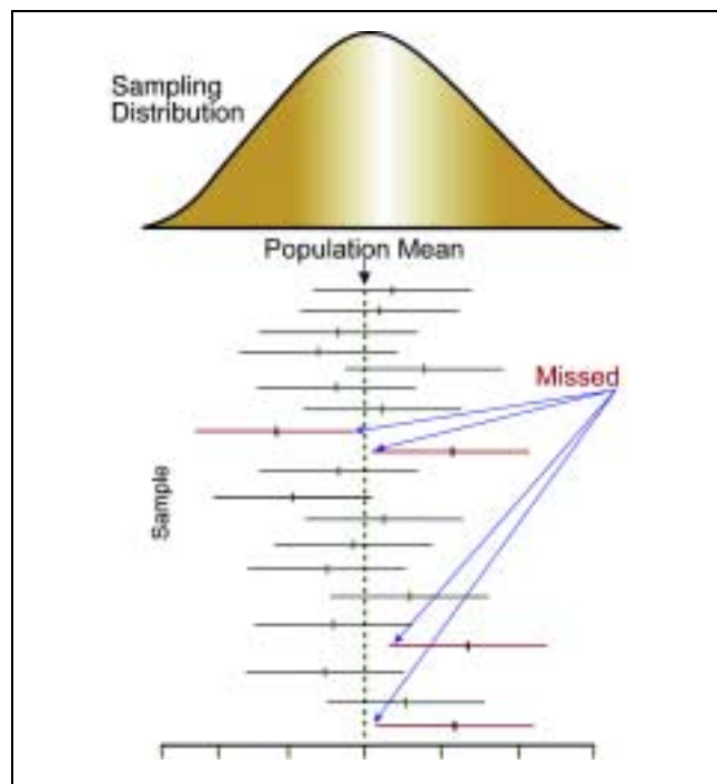
Figure 6. 80% confidence intervals.
