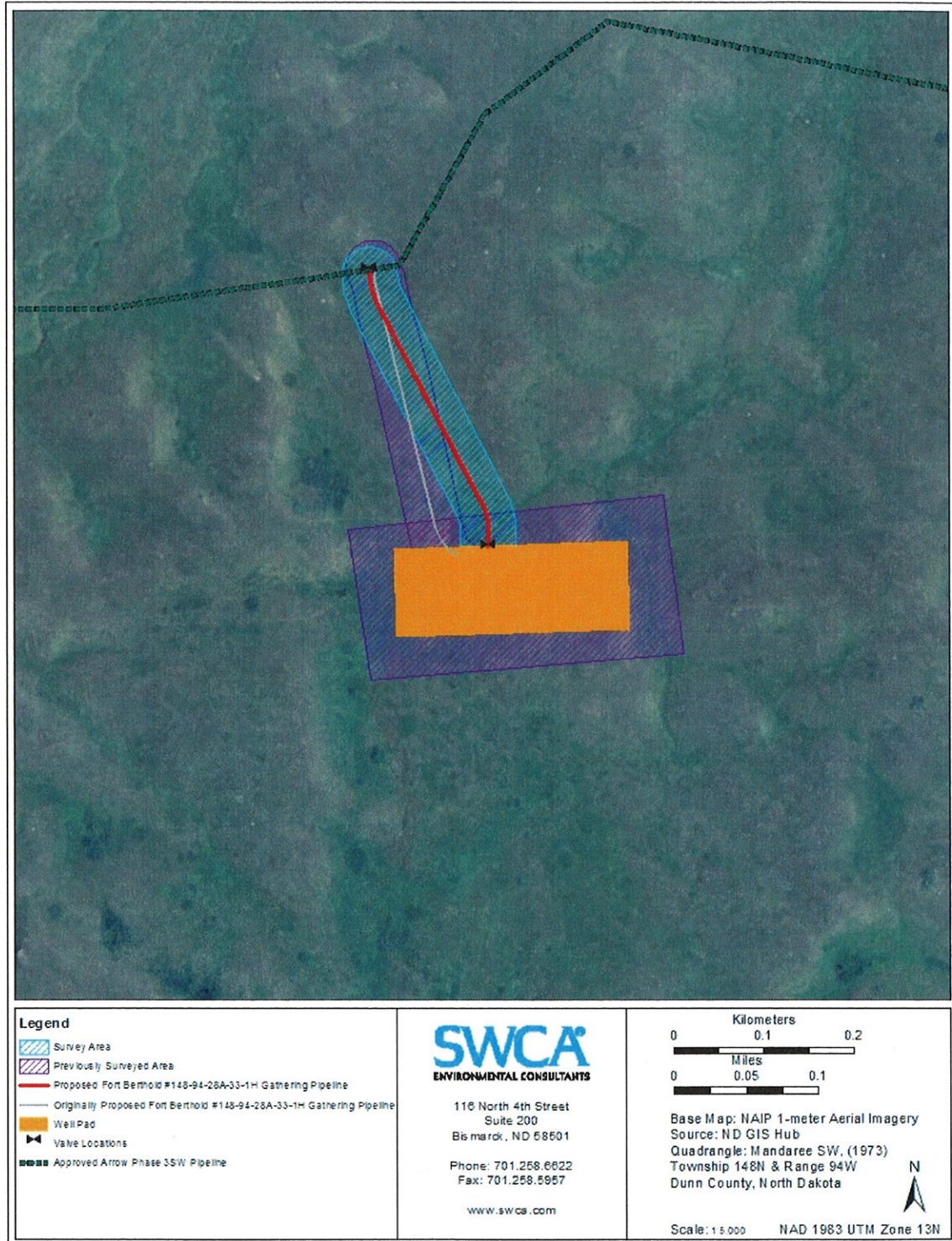
Figure 1. Proposed FB #148-94-28A-33-1H & #148-94-28A-33-2H Gathering Pipeline Alignment
