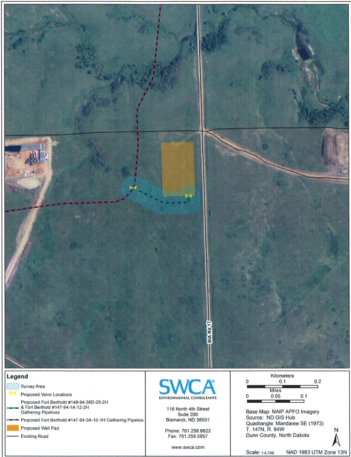
Figure 1. FB #148-94-36D-25-2H & #147-94-1A-12-2H gathering pipeline alignment
