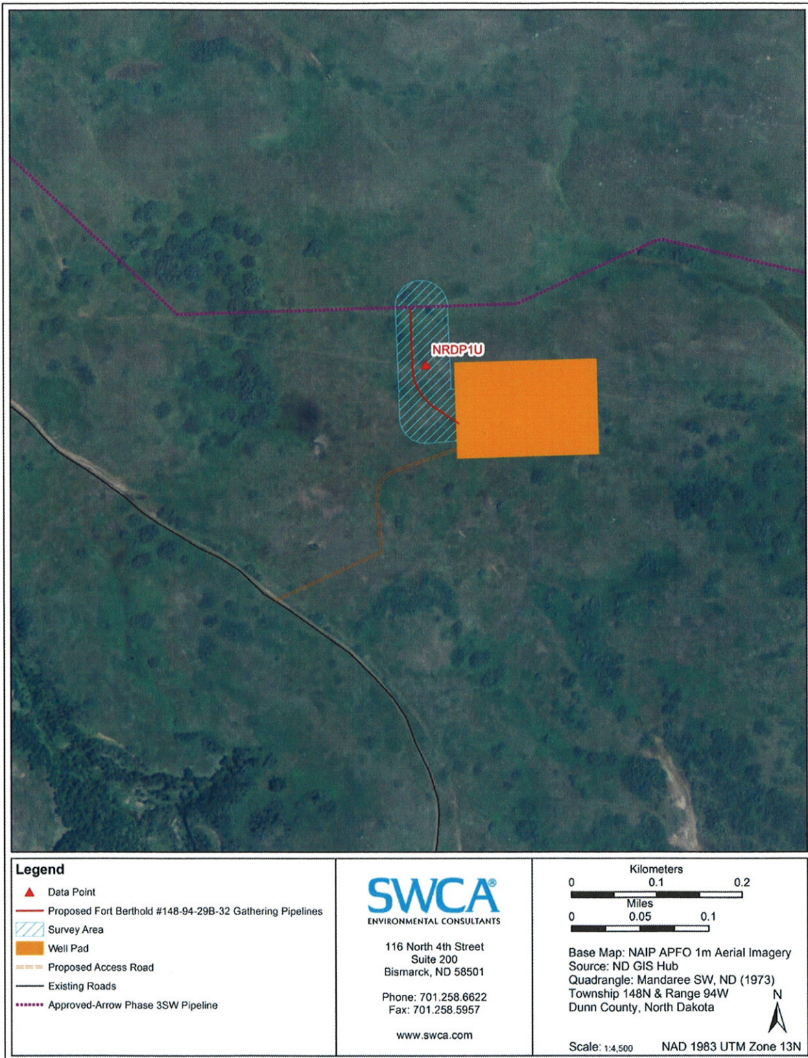
Figure 1. Proposed Fort Berthold #148-94-29B-32-1H, -2H, -3H gathering pipeline alignment
