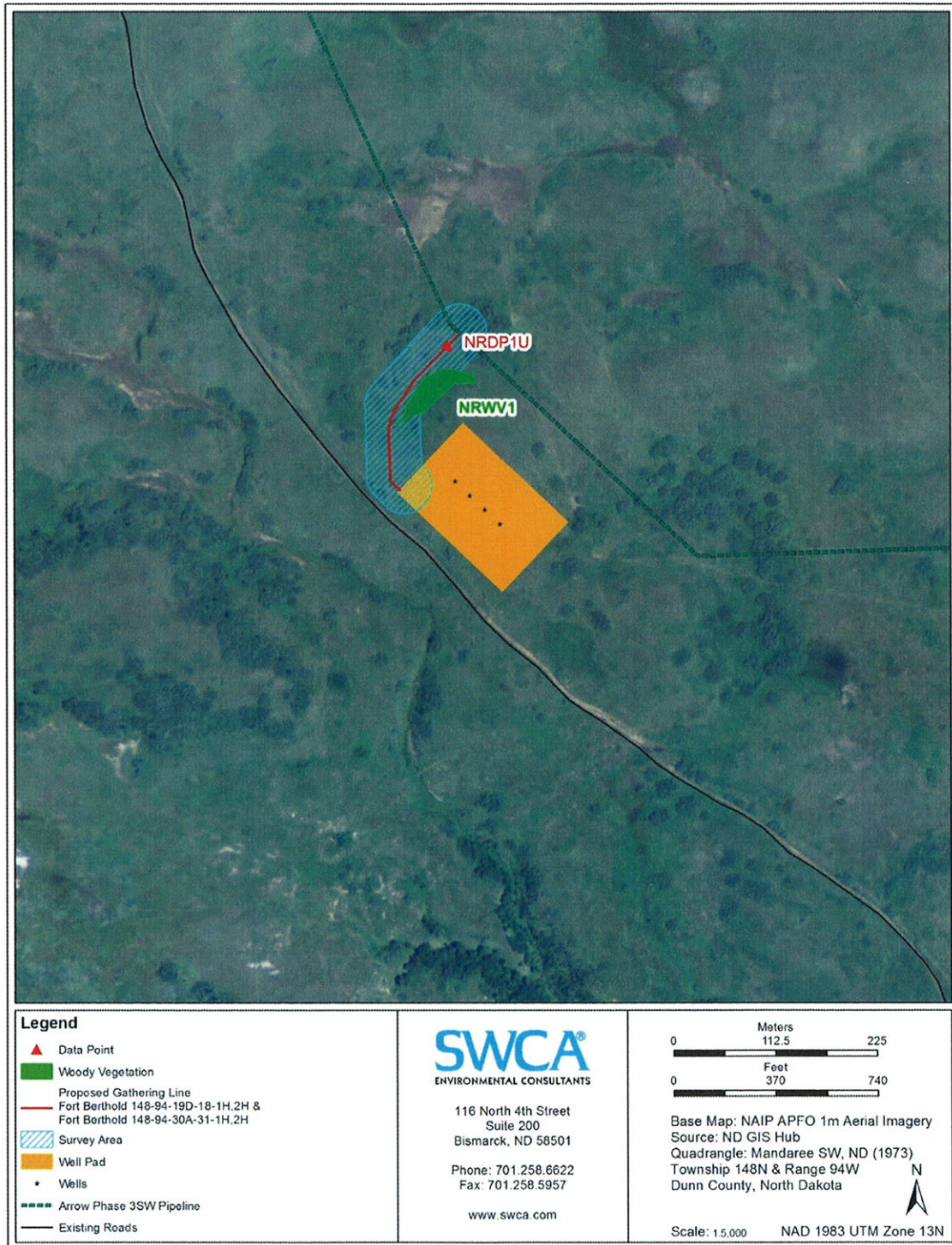
Figure 1. Proposed FB #148-94-19D-18-1H, -2H & #148-94-30A-31-1H, -2H gathering pipeline alignment
