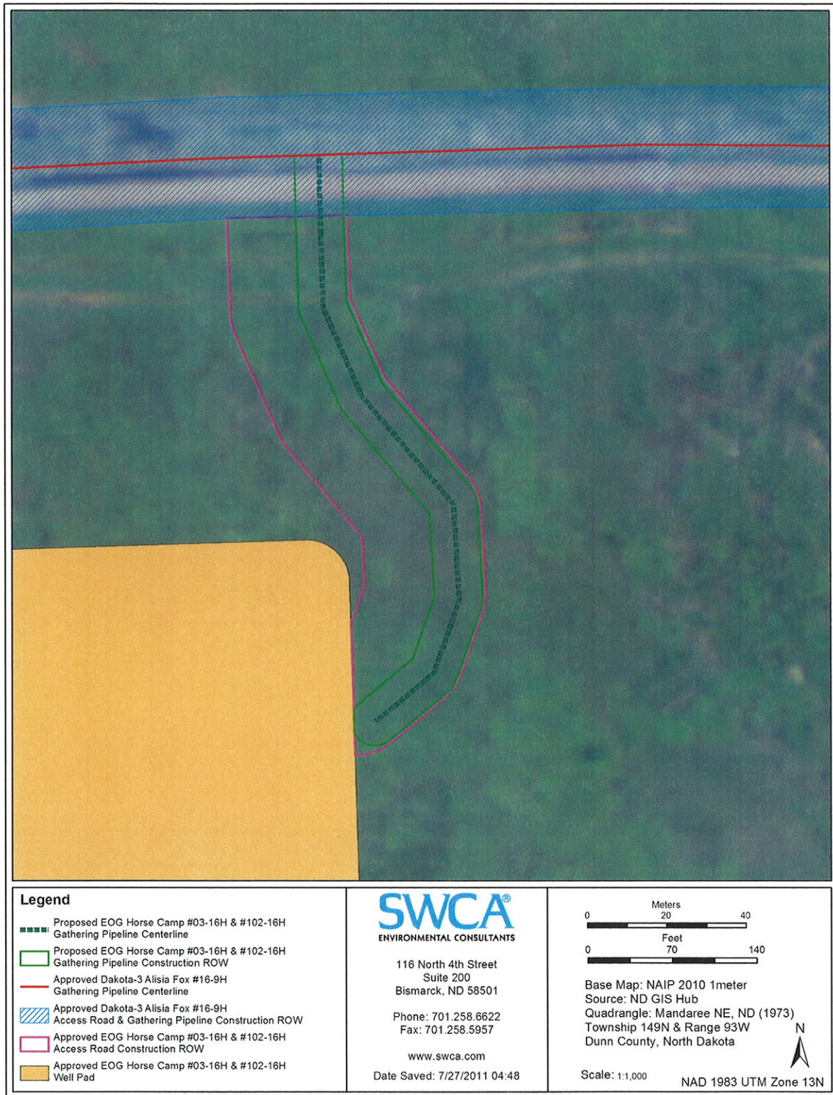
Figure 1. Map of the proposed Horse Camp #03-16H/Horse Camp #102-16H Gathering Pipeline System.
