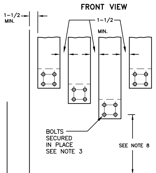
FIGURE 5 REQUIREMENTS FOR BOTTOM STAGGER MINIMATING FACILITIES
