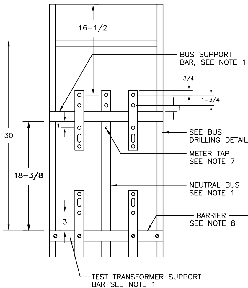
FRONT VIEW
