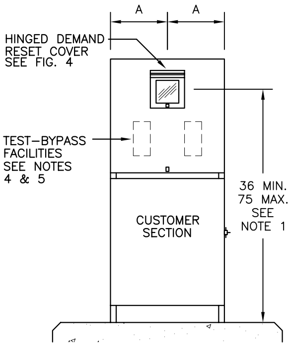
FIGURE 1 FRONT VIEW
