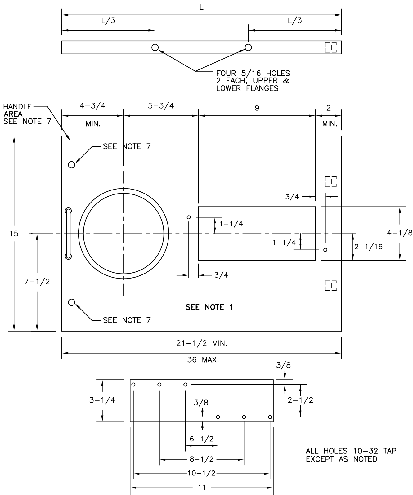
TEST SWITCH MOUNTING ALL DIMENSIONS SHOWN ARE IN INCHES
