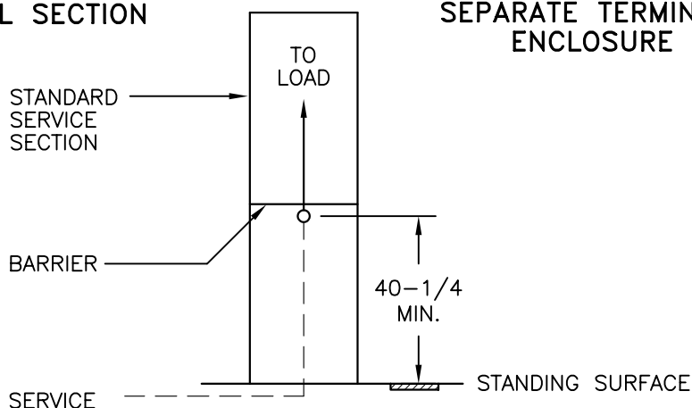
FIGURE 3 2000 AMP MAXIMUM BOTTOM FEED PULL SECTION
