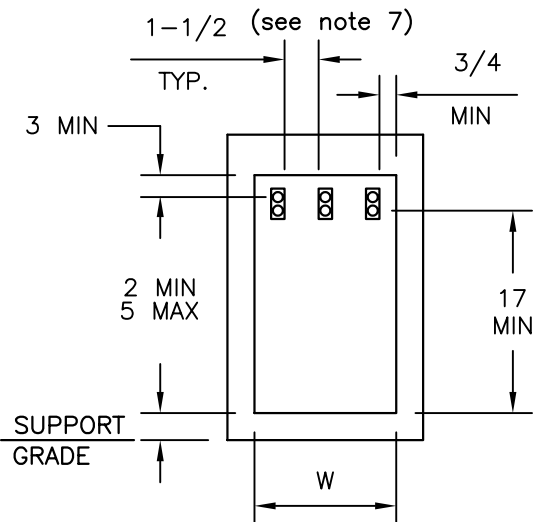
FIGURE 3 WIREWAY PULL SECTION
