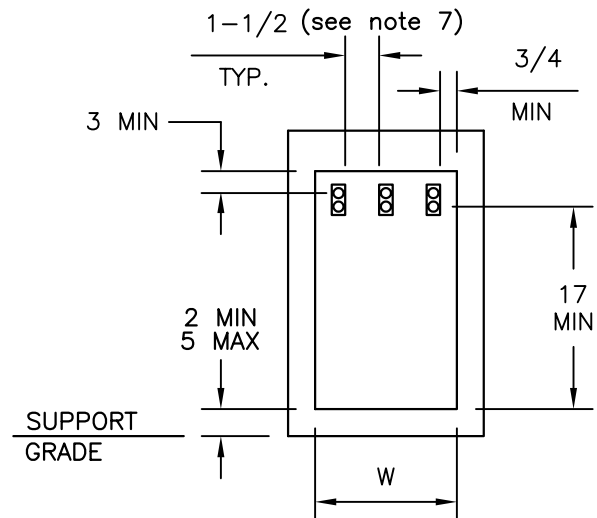
FIGURE 3 WIREWAY PULL SECTION
