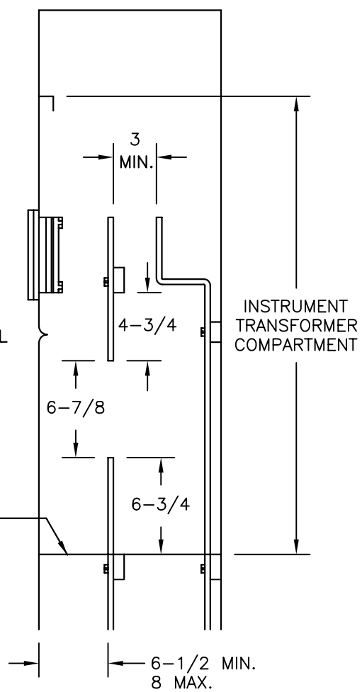
SIDE VIEW
