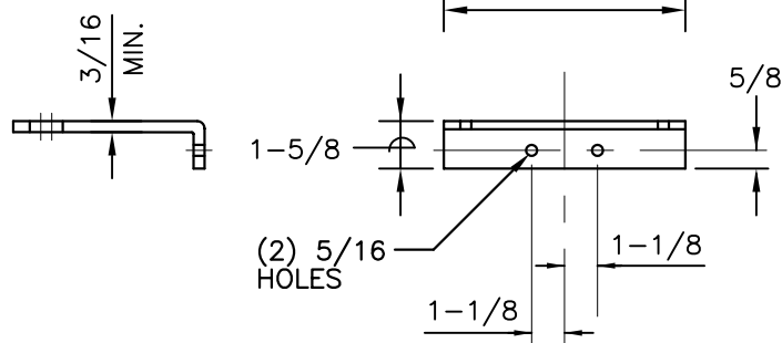
DETAIL "C" INSULATED SUPPORT FOR CURRENT TRANSFORMER (MATERIAL: INSULATING, NON-TRACKING)
