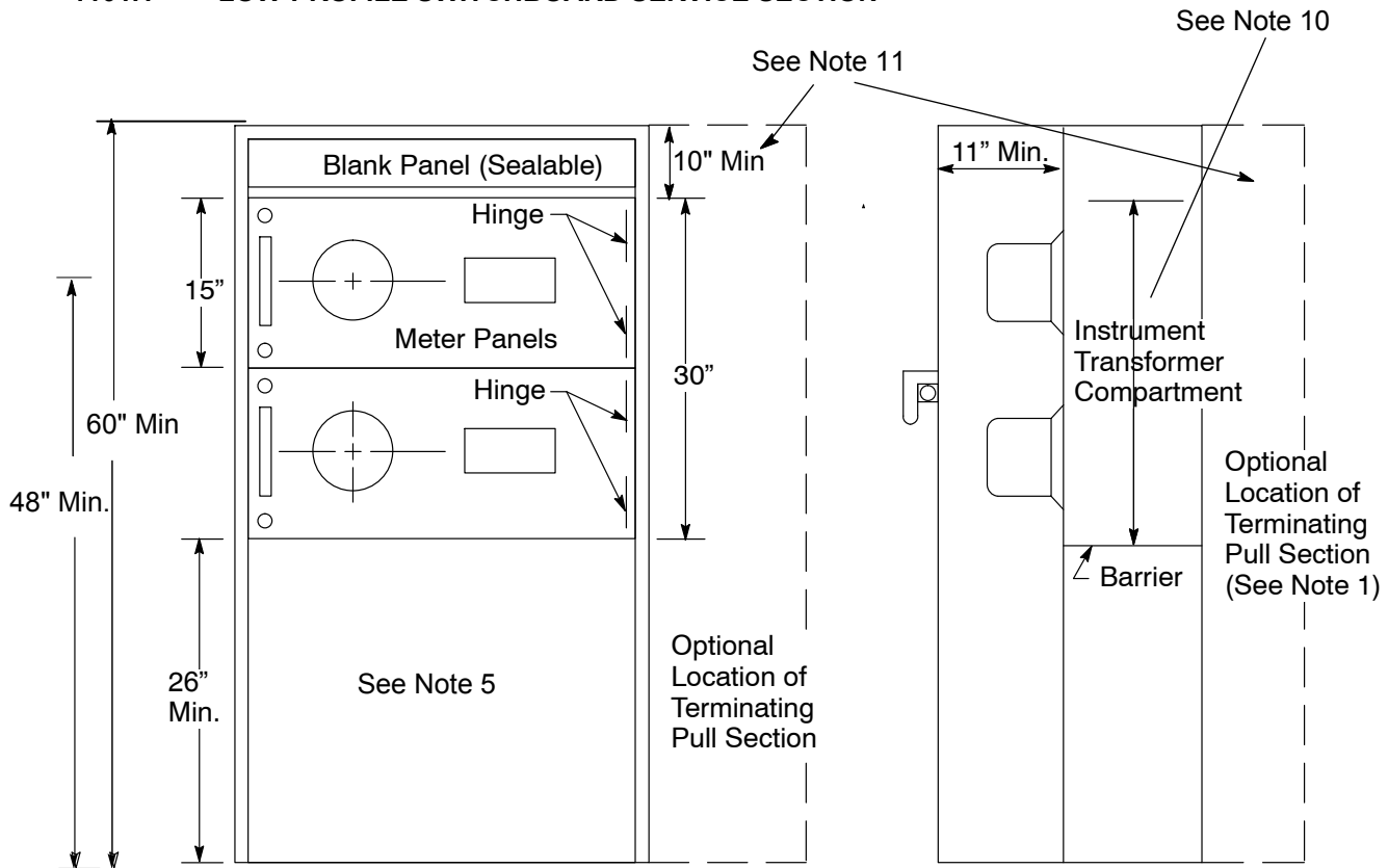
CRA-ES DWG. 1101.1 ALL DIMENSIONS SHOWN ARE IN INCHES
