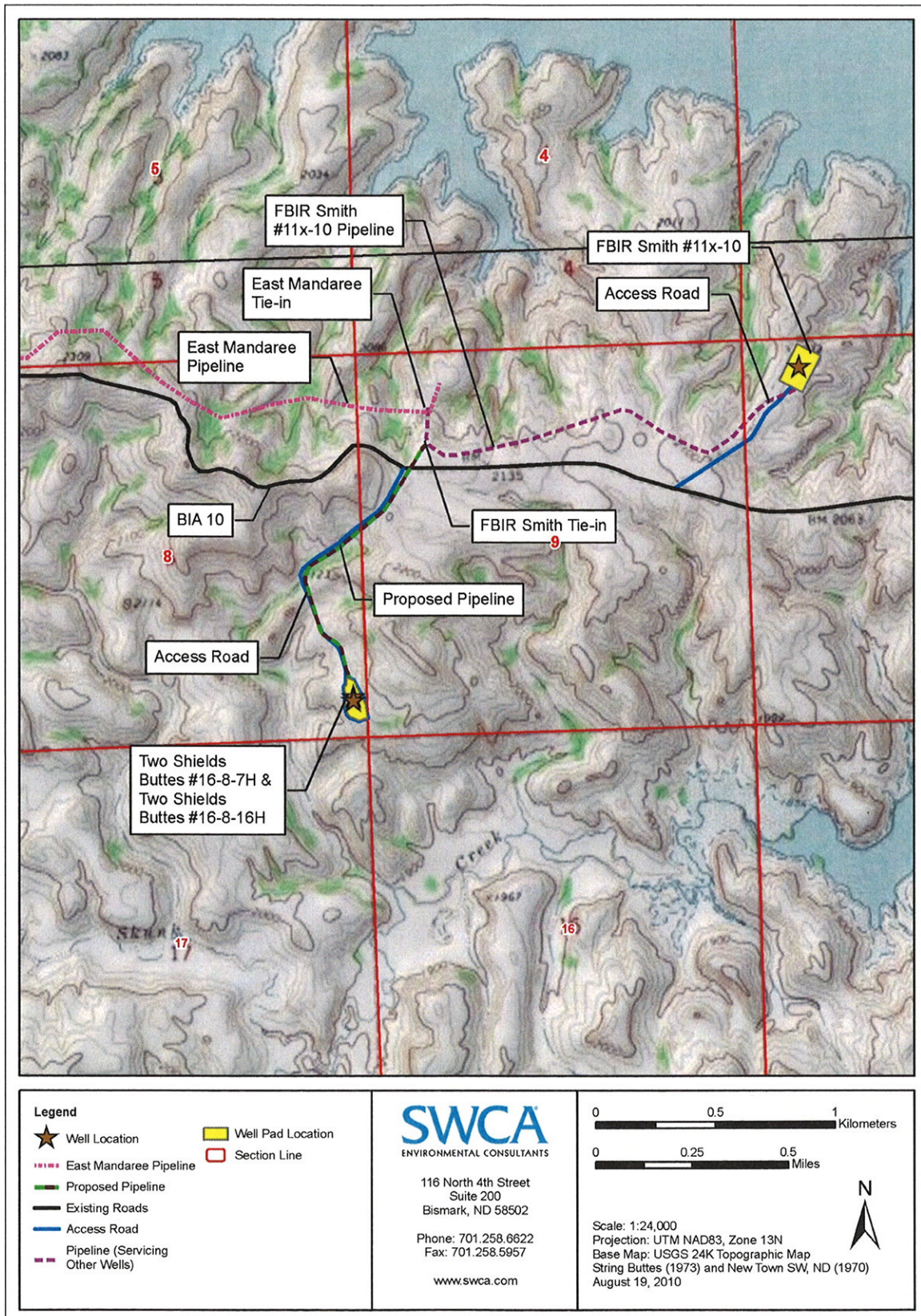
Figure 1. Proposed Two Shields Butte #16-8-7H and Two Shields Butte #16-8-16H gathering pipelines and associated well pad.
