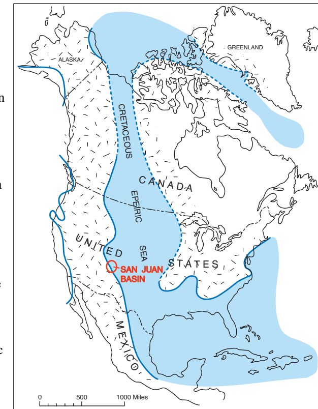
Figure J-8. Probable configuration of the North American Epicontinental Seaway at the time the Upper Cretaceous rocks of the San Juan Basin accumulated (after Fassett, 1988, p. 26).
